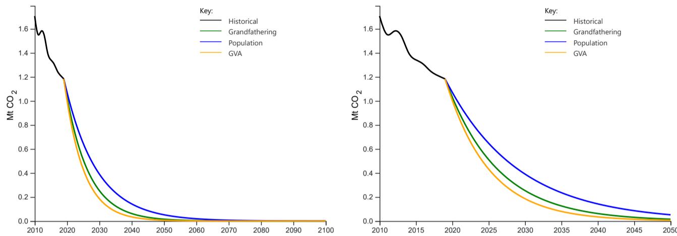
Figure 3a (left): Energy related CO 2 only emissions pathways (2010-2100) for Wirral premised on carbon budgets shown in Table 2. Figure 3b (right): Energy related CO 2 only emissions pathways (2010-2050) for Wirral premised on carbon budgets shown in Table 2. y-axis shows emissions in MtCO 2
