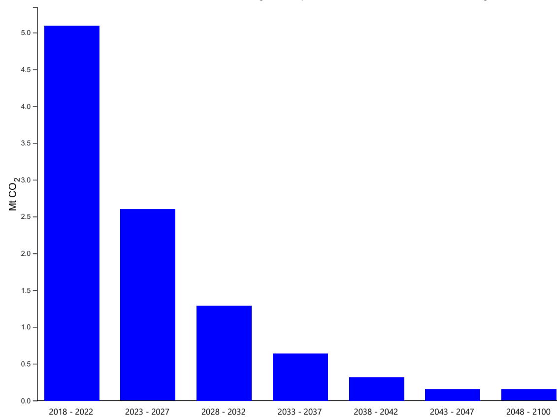
Figure 2: Cumulative CO 2 emissions for budget period (based on Table 1) from 2018 to 2100 for Wirral
