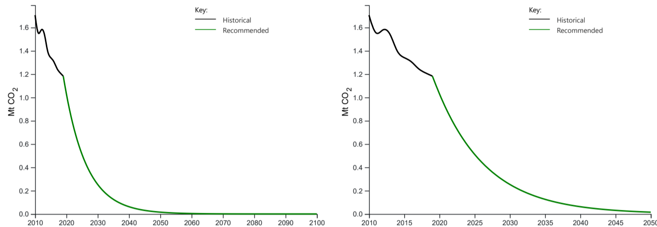
Figure 1a (left): Energy related CO 2 only emissions pathways (2010-2100) for Wirral premised on the recommended carbon budget. Figure 1b (right): Energy CO 2 only emissions pathways (2010-2050) for Wirral premised on the recommended carbon budget. y-axis shows emissions in MtCO 2
