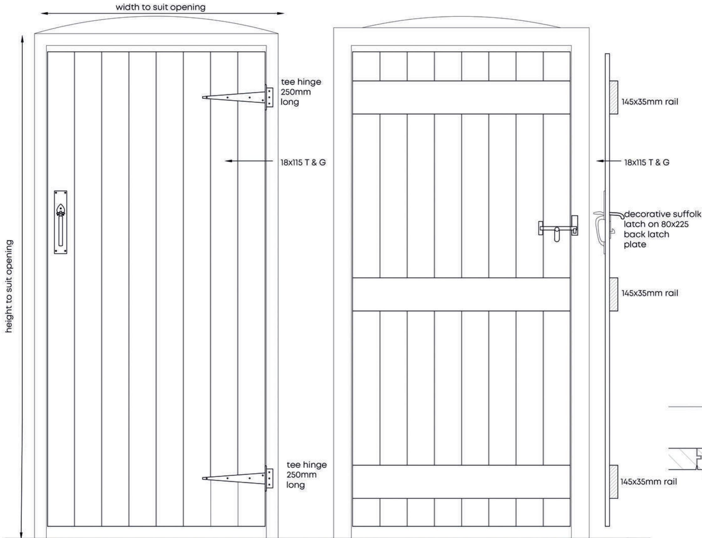
External Elevation 1:10
