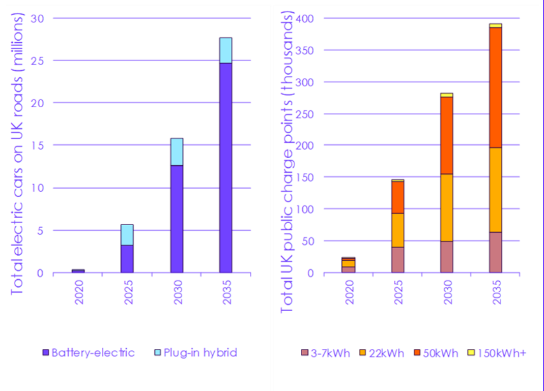
Figure 3.1.b Total electric cars on the road and supporting charging infrastructure in the Balanced Net Zero Pathway
